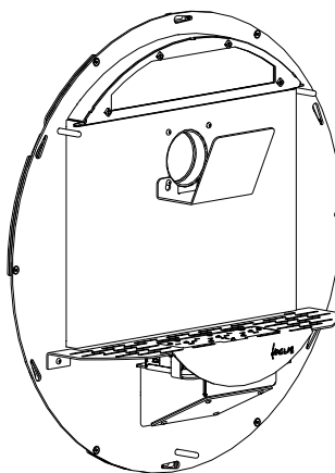
RESTRICTOR A
